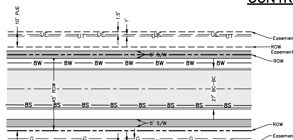
5' P.A.E. | 11.5' | 45' R.O.W. | 11.5' | 5' P.A.E. 2.5' | 5' | 4' | 13.5' | 4' | 5' | 2.5' 2" HMA 3% 3% 2' Laydown Curb 6" Crushed Limestone Base 6" Stabilized Subgrade (Material & Rate to be determined by material testing during construction) 2" Sidewalk 4:1 4:1 27' B.C.-B.C.
